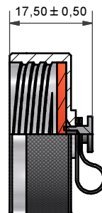
100P160-17-1-C-EO EYELET ONLY VERSION (NO LANYARD)
