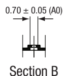
Figure 12. SOD-882 Tape and Reel Dimensions
