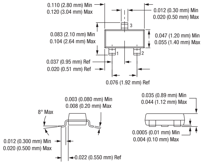
Figure 9. SOT-23 Package Dimension Drawing
