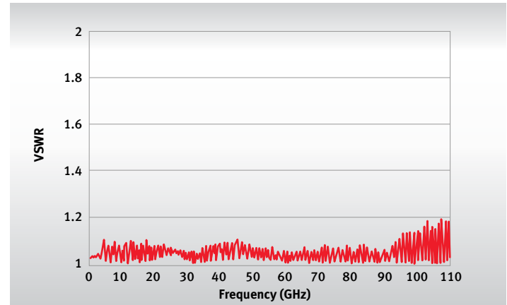
FIGURE 3: TYPICAL VSWR 1
