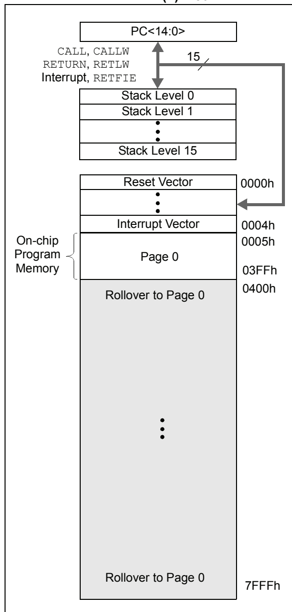
FIGURE 3-1: PROGRAM MEMORY MAP AND STACK FOR PIC12(L)F1501
