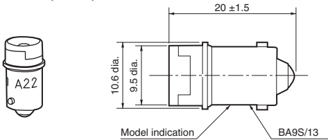
Lamp LED A22-6□, 12□, 24□
