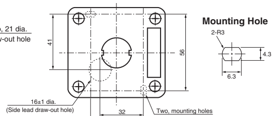
Cable Draw-out Hole (Top View)
