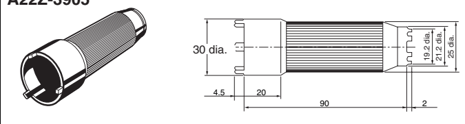
Tightening Tool A22Z-3905
