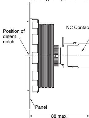
Mounting a 1-pole Switch Unit *
