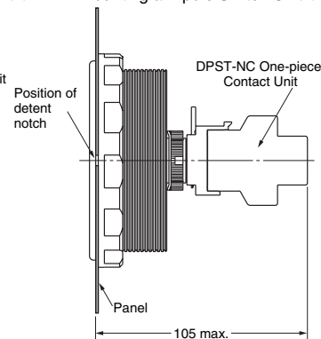
Mounting a 2-pole Switch Unit *
