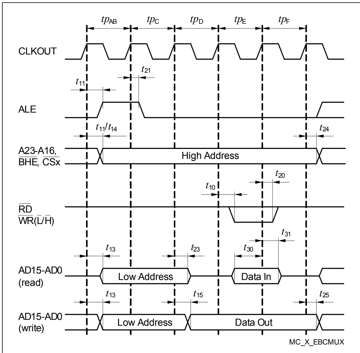
Figure 22 Multiplexed Bus Cycle
