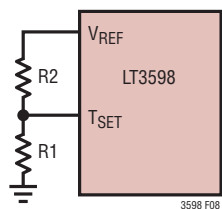
Figure 8. Programming the T SET Pin
