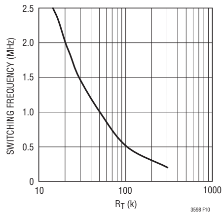
Figure 10. Switching Frequency
