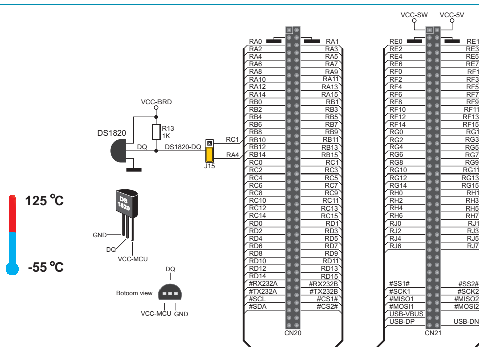
Figure 10-4: DS1820 and microcontroller connection schematic
