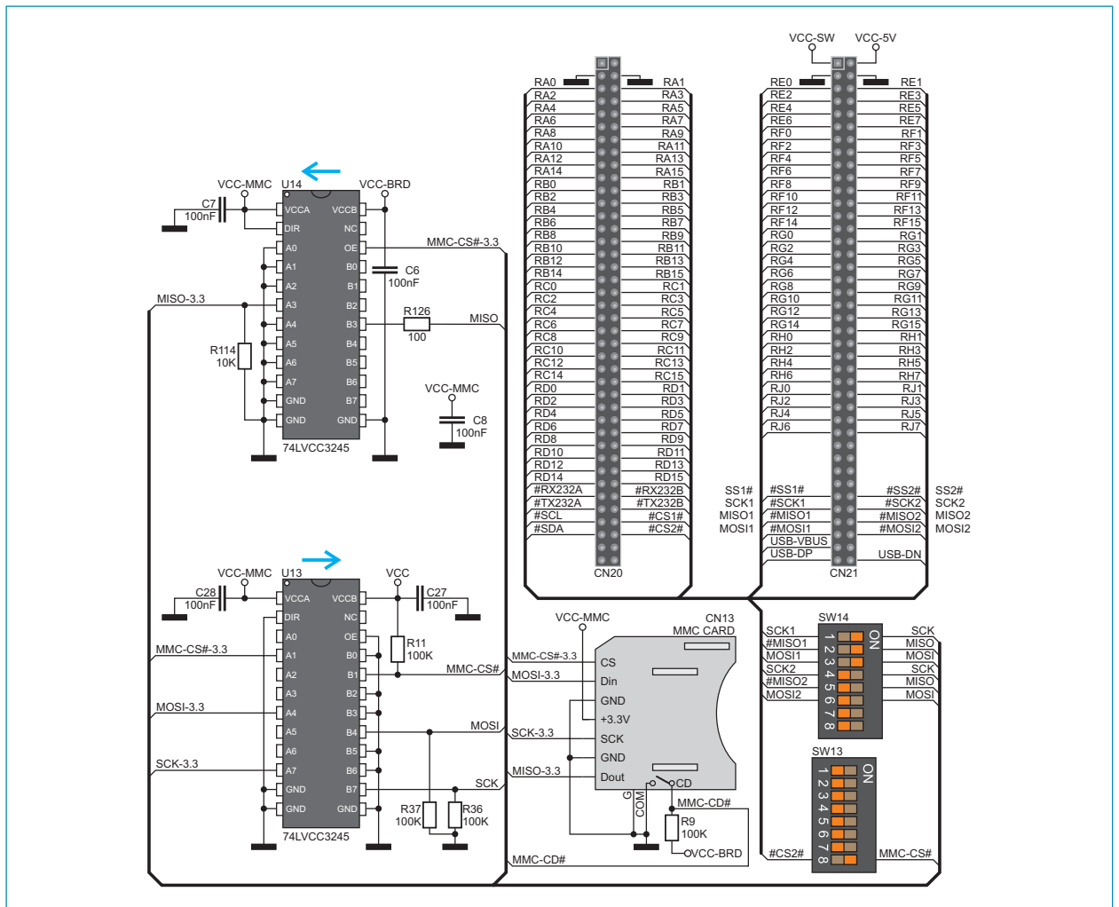
Figure 11-1: MMC/SD memory card
