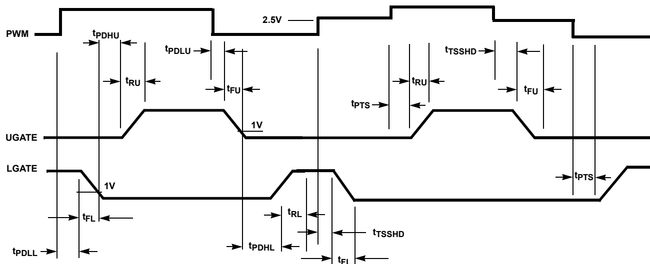
FIGURE 3. TIMING DIAGRAM
