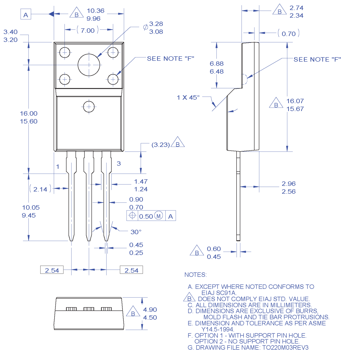
Figure 16. TO220, Molded, 3-Lead, Full Pack, EIAJ SC91, Straight Lead
