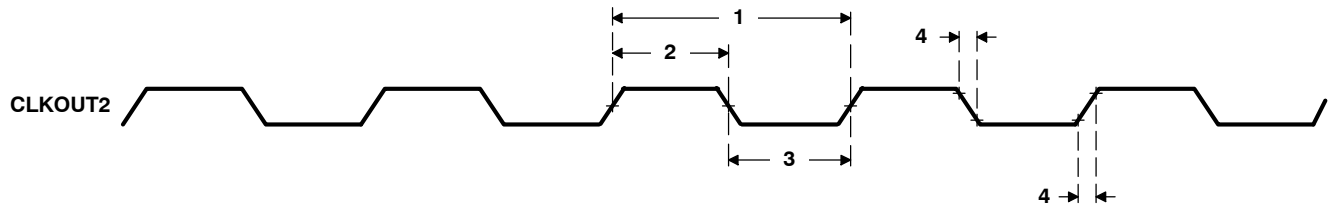
Figure 22. CLKOUT2 Timings
