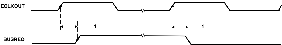
Figure 38. BUSREQ Timing
