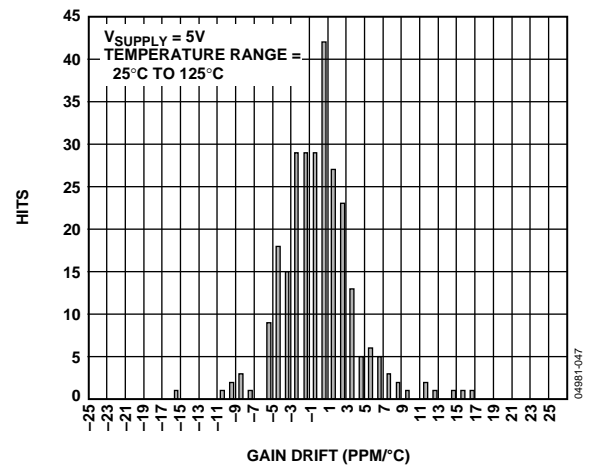
Figure 39. Gain Drift Distribution, SOIC, Temperature Range = 25^{\circ}\text{C} to 125^{\circ}\text{C}
