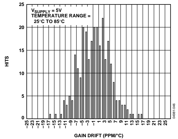
Figure 38. Gain Drift Distribution, SOIC, Temperature Range = 25^{\circ}\text{C} to 85^{\circ}\text{C}
