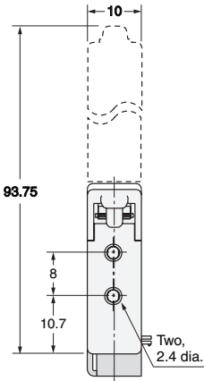
Mounting Holes
