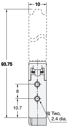
Mounting Holes
