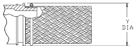
TINEL-LOCK TERMINATION
