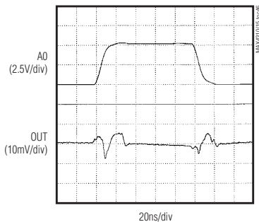
CHANNEL-SWITCHING TRANSIENT
