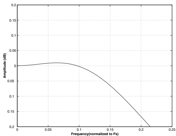
Figure 38. Quad-Speed (fast) Passband Ripple
