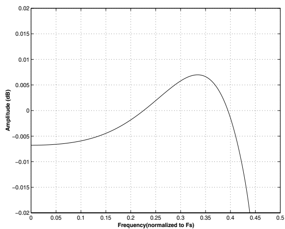
Figure 26. Single-Speed (slow) Passband Ripple
