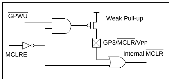
FIGURE 8-1: \overline{\text{MCLR}} SELECT
