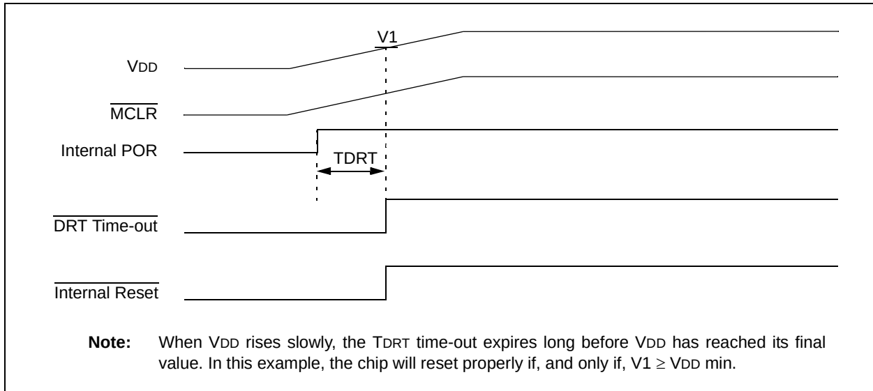
FIGURE 8-5: TIME-OUT SEQUENCE ON POWER-UP ( \overline{\text{MCLR}} TIED TO V_{DD} ): SLOW V_{DD} RISE TIME
