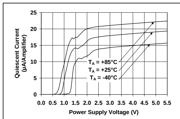
FIGURE 2-19: Quiescent Current vs. Power Supply Voltage.
