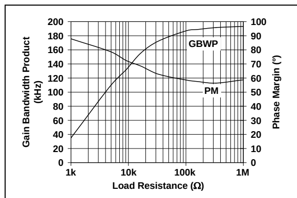
FIGURE 2-21: Gain-Bandwidth Product, Phase Margin vs. Load Resistance.
