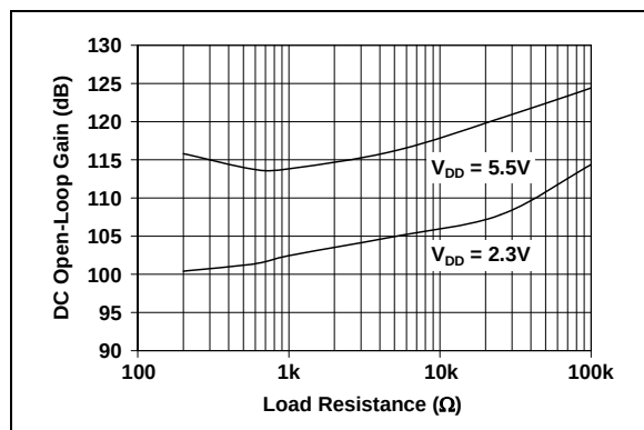
FIGURE 2-20: DC Open-Loop Gain vs. Load Resistance.
