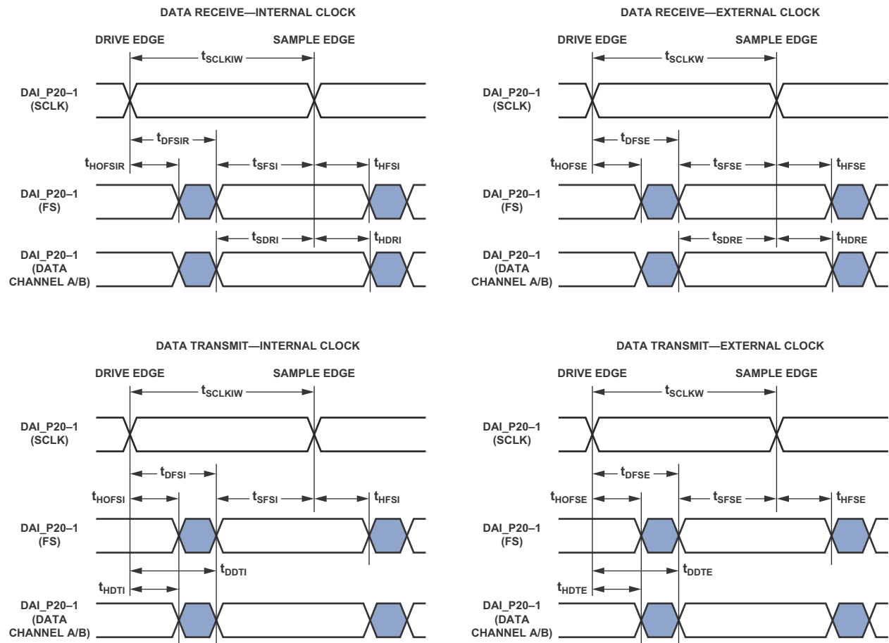
Figure 22. Serial Ports
