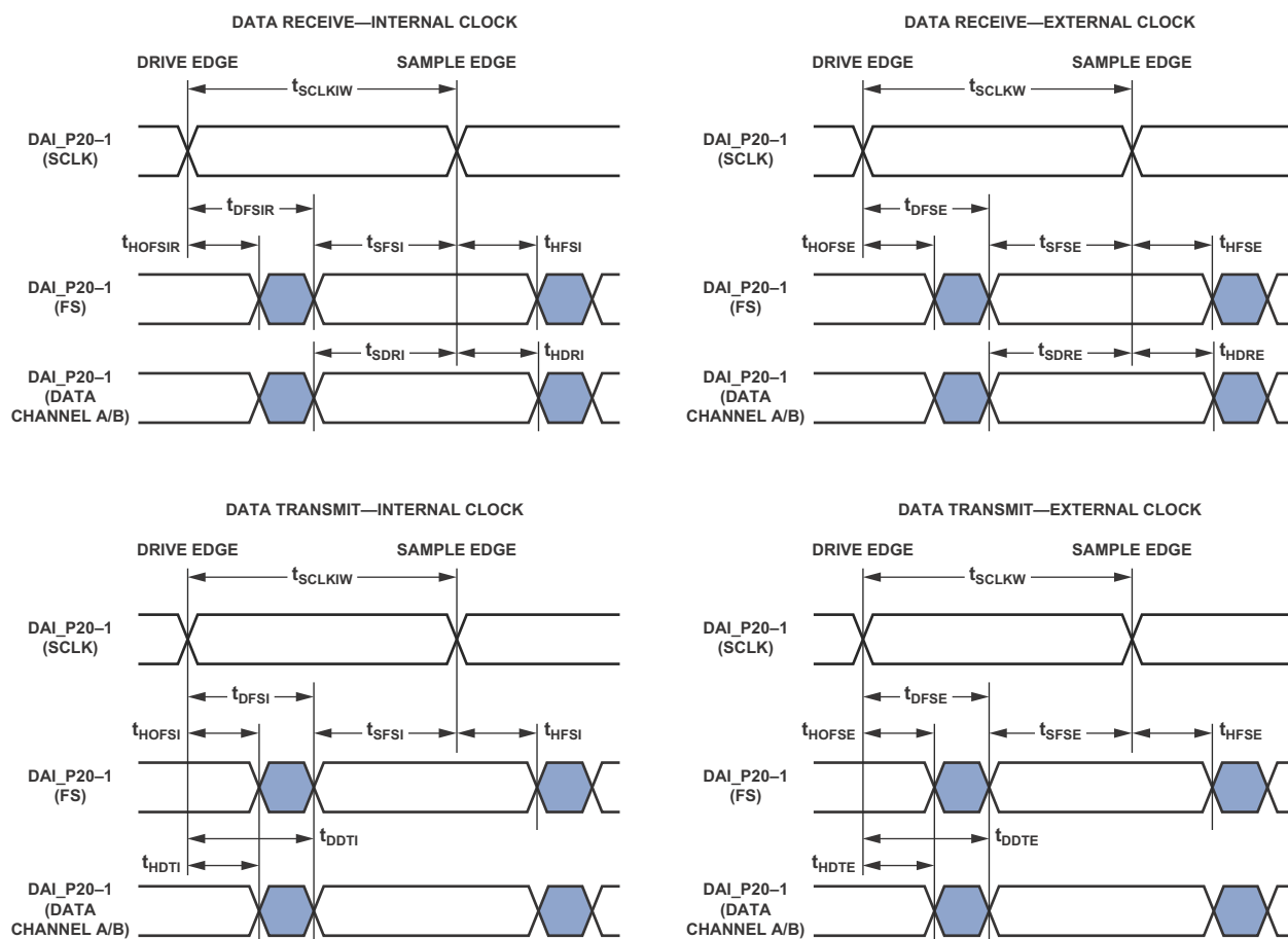
Figure 22. Serial Ports
