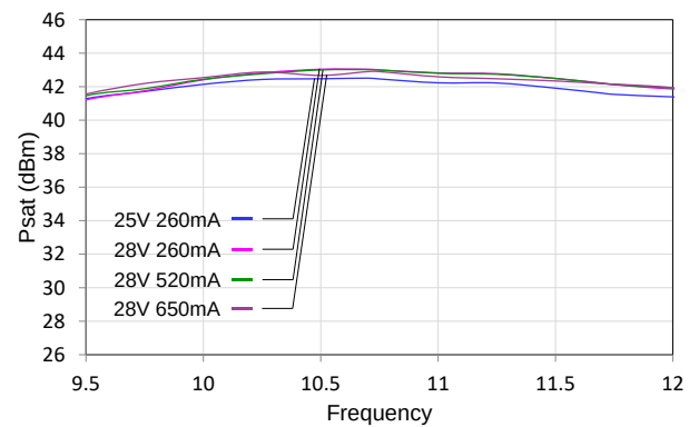
Psat vs. Frequency vs. Bias (Vd3)
