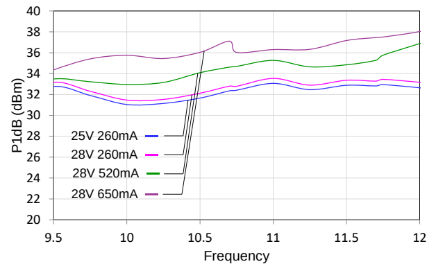
P1dB vs. Frequency vs. Bias (Vd3)
