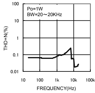
Fig. 17 THD+N - Frequency
