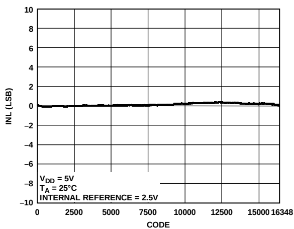
Figure 16. AD5685R INL
