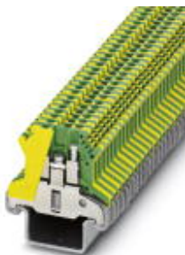
Ground modular terminal block, Connection method: Screw connection, Cross section: 0.2 mm 2 - 4 mm 2 , AWG 24 - 12, Width: 5.2 mm, Color: green-yellow, Mounting type: NS 35/15-2,3
