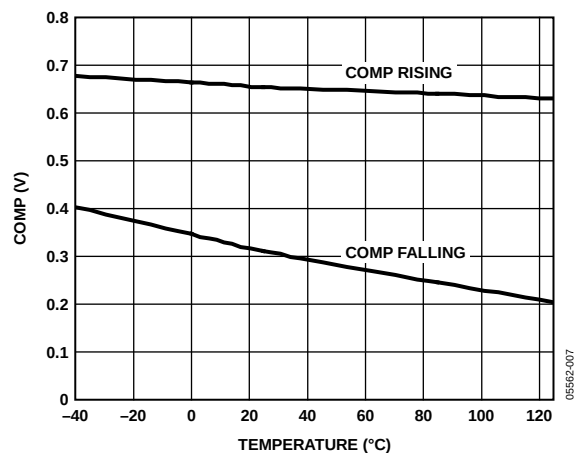
Figure 6. COMP Shutdown Threshold vs. Temperature
