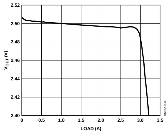
Figure 7. Typical Load Regulation ( V_{IN} = 5V ; See Figure 1)
