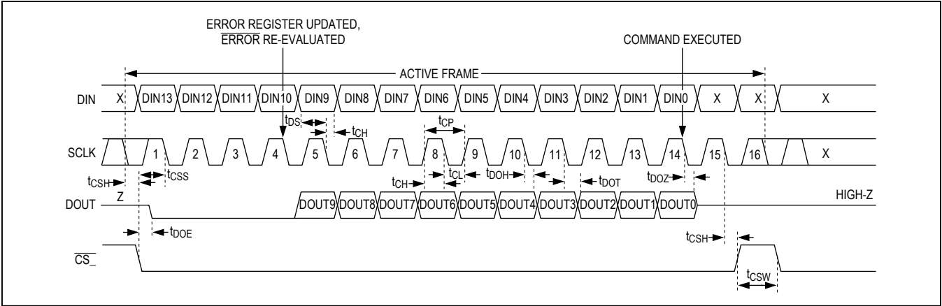
Figure 8. Minimum SPI Programming Operation (Typically for Single Device Applications)
