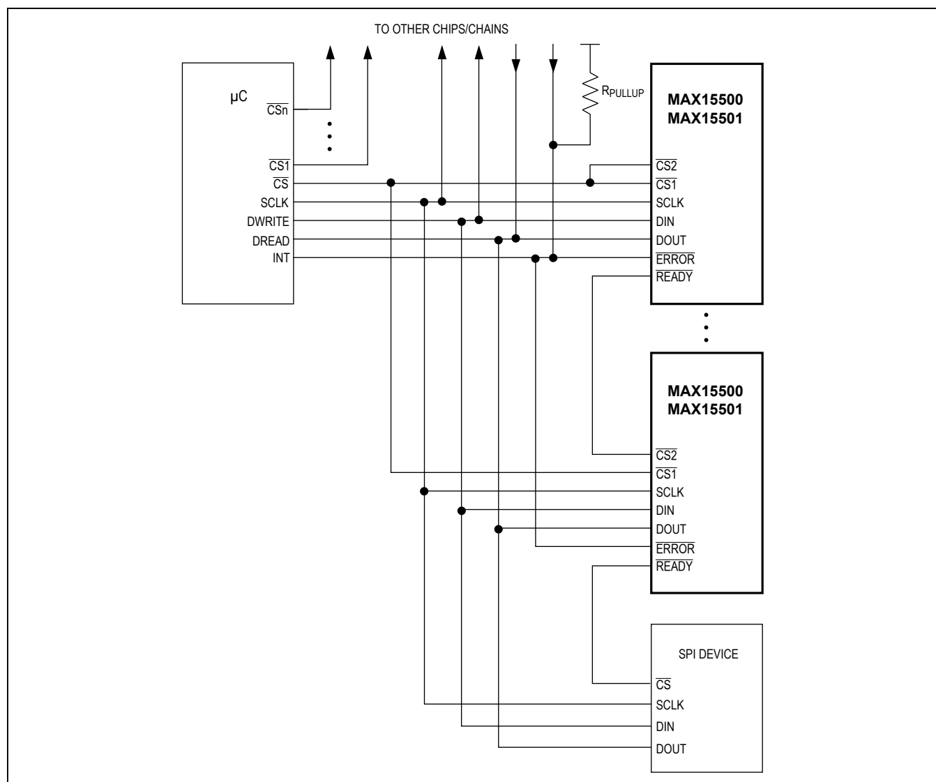
Figure 6. Daisy-Chain Terminating (Compatible with Standard SPI)
