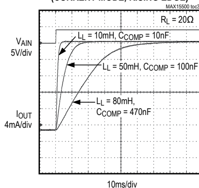
LARGE-SIGNAL SETTLING TIME (CURRENT MODE, RISING EDGE)
