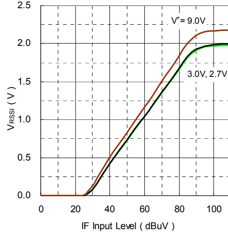
RSSI Output versus IF Input Level and Supply Voltage
