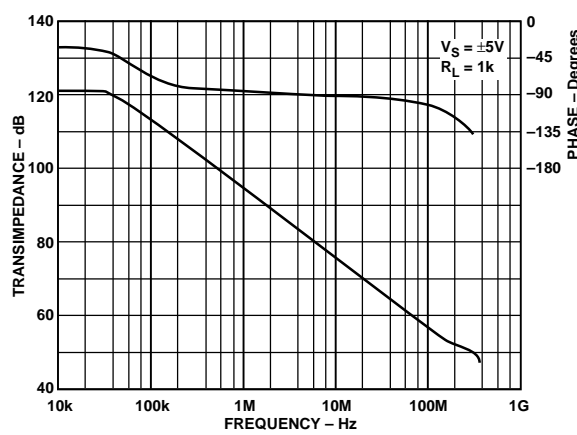
Figure 14. Open-Loop Transimpedance vs. Frequency (Relative to 1 \Omega )
