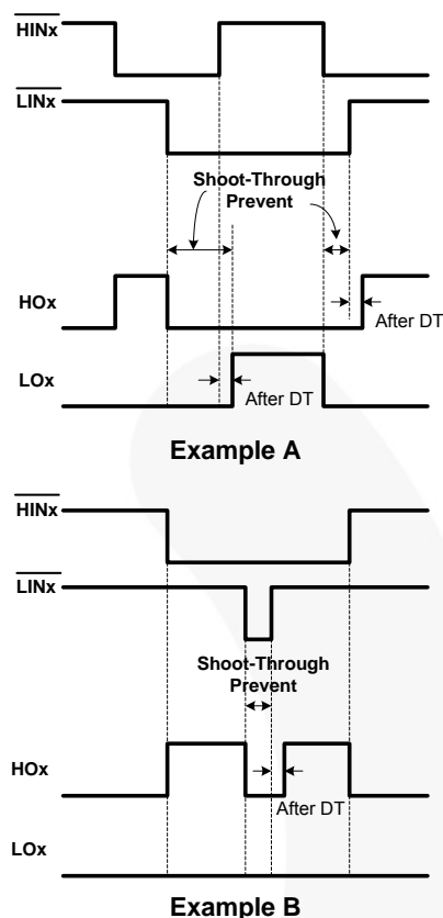
Figure 39. Shoot-Through Protection
