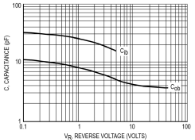
Capacitances
