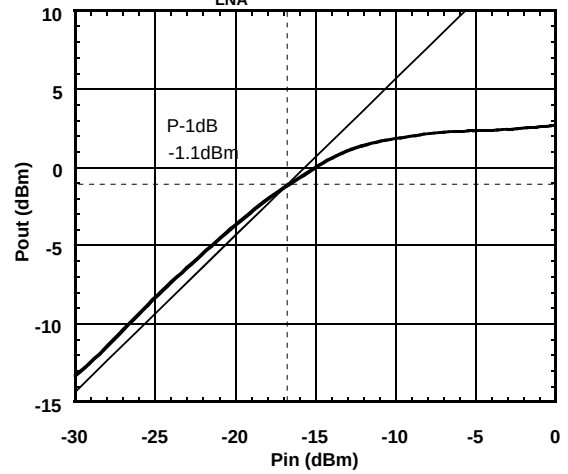
Pout vs. Pin ( V_{LNA}=2.7\text{V}, f=820\text{MHz} )
