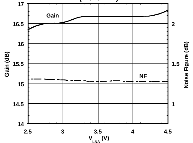
Gain, Noise Figure vs. V_{LNA} ( f=820\text{MHz} )
