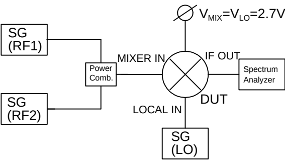
IF,IM3 Measuring Block Diagram
