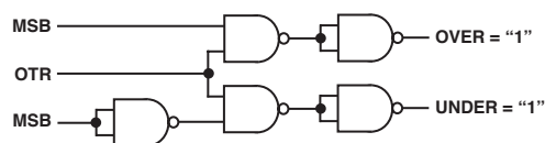
Figure 23. Overrange or Underrange Logic
