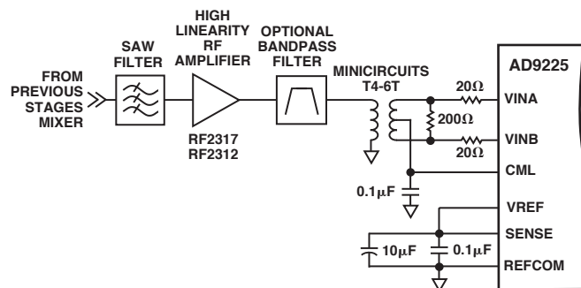
Figure 26. Example of AD9225 IF Sampling Circuit
