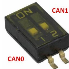
Figure 44: CAN Termination Switch
