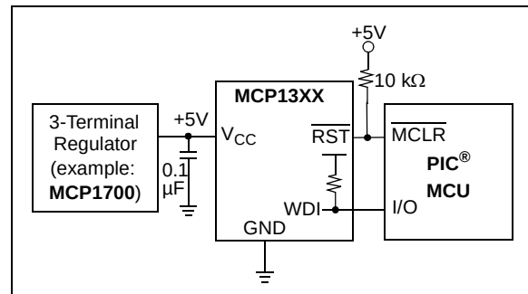
FIGURE 4-19: Watchdog Timer.
