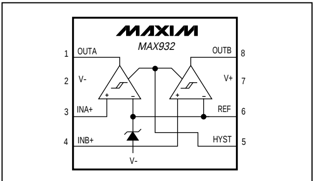
Figure 1a. MAX932 Functional Diagram
