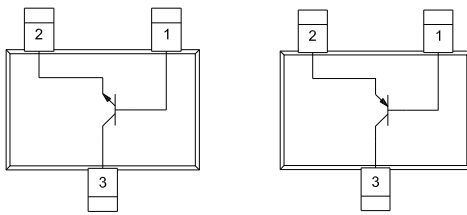
CMST3904 NPN
