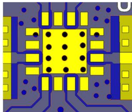
Mounting Pad Details
