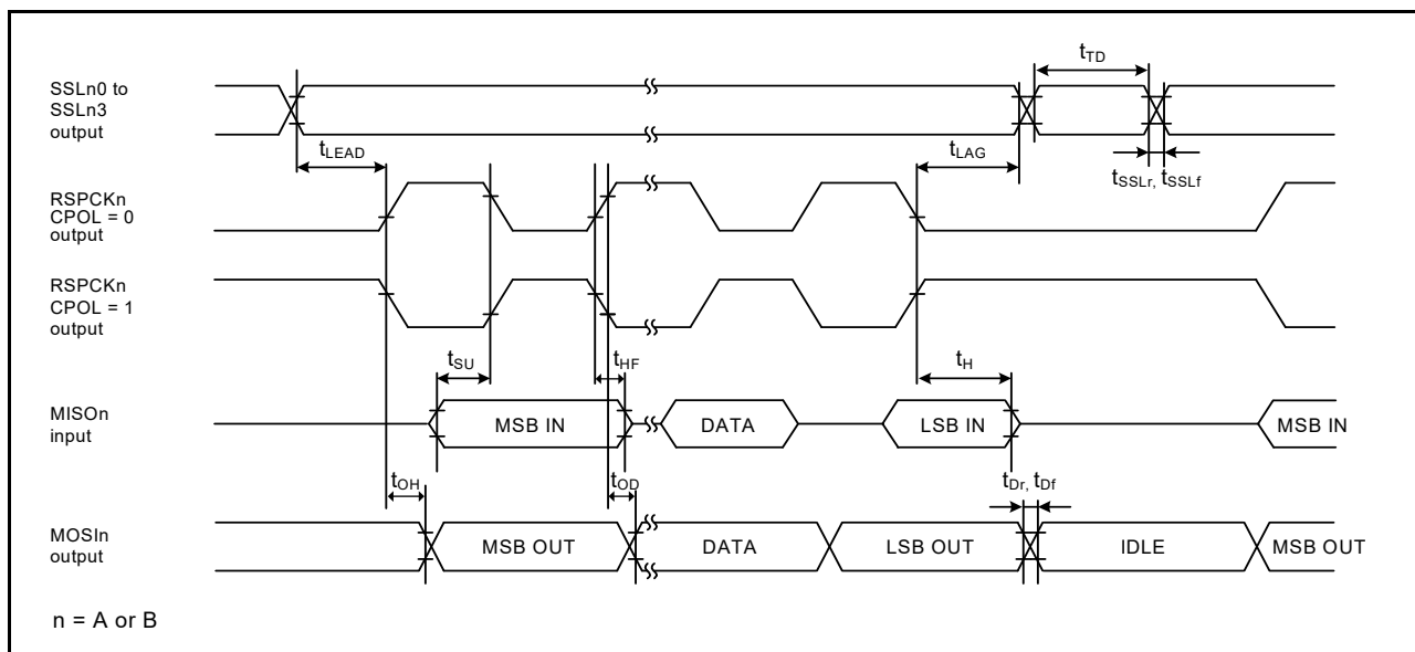
Figure 2.53 SPI timing (master, CPHA = 1) (bit rate: PCLKB division ratio is set to 1/2)
