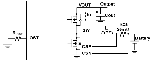
Figure 12. Boost output current setting circuit
