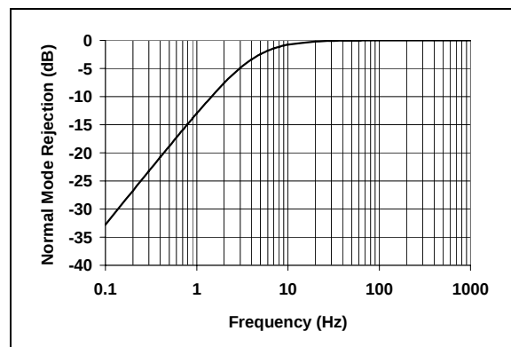
FIGURE 4-4: HPF Magnitude Response ( \text{MCLK} = 3.58\text{ MHz} ).
