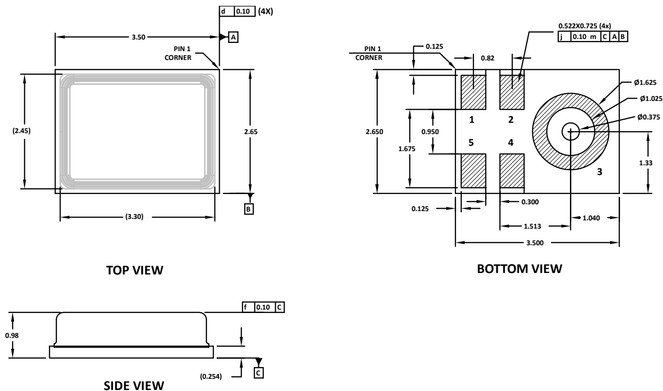
Figure 16. 5-Terminal Chip Array Small Outline No Lead Cavity [LGA_CAV]
