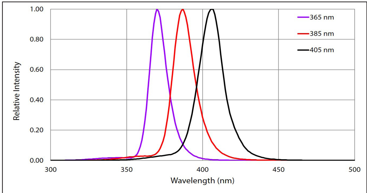
Typical Spectrum 9
