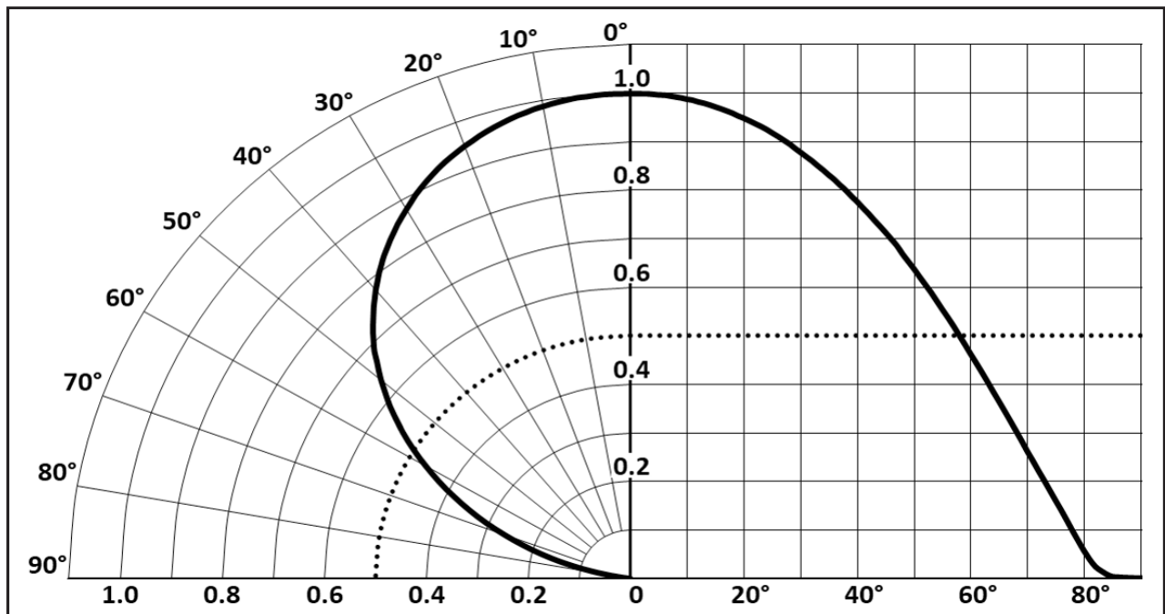
Radiation Pattern 10
