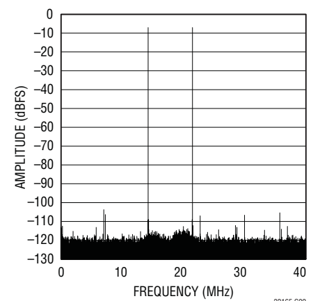
LTC2216 64k Point 2-Tone FFT, f_{IN} = 14.25\text{MHz} and 21.5\text{MHz} , -7dBFS
