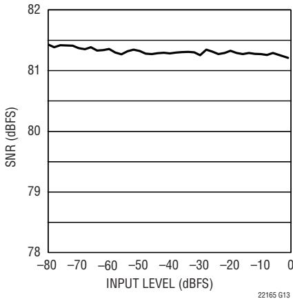
LTC2216 SNR vs Input Level, f_{IN} = 15.2\text{MHz}
