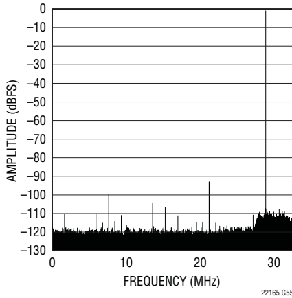
LTC2215 64k Point FFT, f_{IN} = 28.7\text{MHz} , -1dBFS
