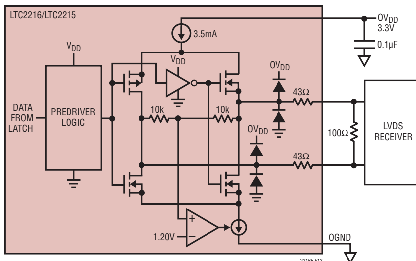
Figure 13. Equivalent Output Buffer in LVDS Mode
