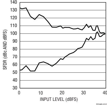
LTC2216 SFDR vs Input Level, f_{IN} = 15.2\text{MHz} , Dither "Off"
