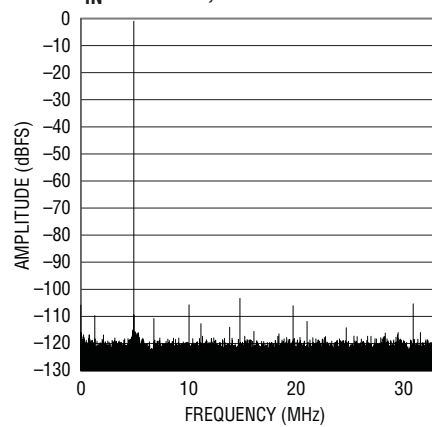
LTC2215 64k Point FFT, f_{IN} = 4.9\text{MHz} , -1dBFS
