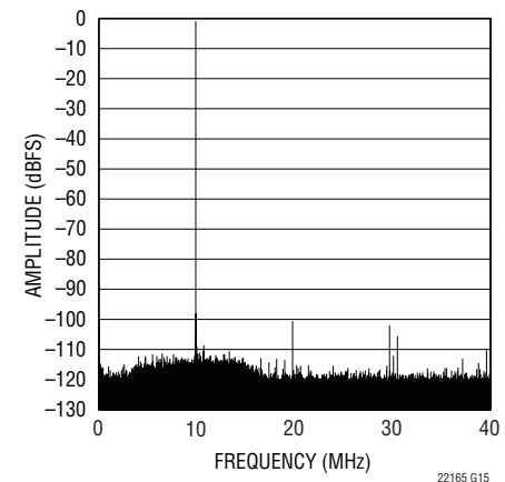
LTC2216 64k Point FFT, f_{IN} = 70.2\text{MHz} , -1dBFS
