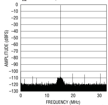
LTC2215 64k Point FFT, f_{IN} = 15.1\text{MHz} , -1dBFS
