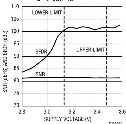
LTC2215 SNR and SFDR vs Supply Voltage ( V_{DD} ), f_{IN} = 5.1\text{MHz}
