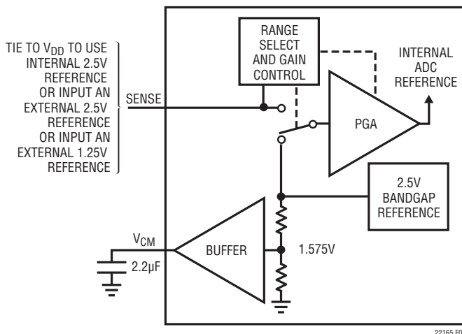
Figure 6. Reference Circuit
