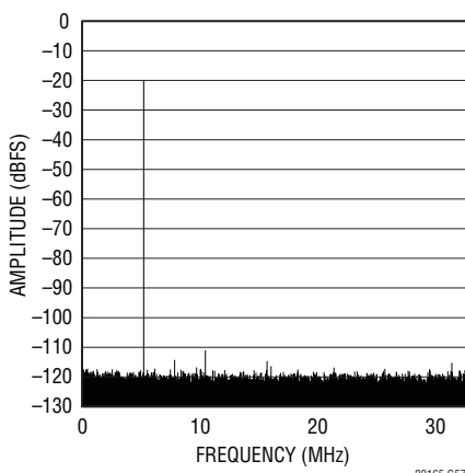
LTC2215 64k Point FFT, f_{IN} = 70.1\text{MHz} , -20dBFS, Dither "Off"
