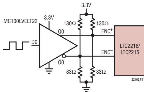
Figure 11. ENC Drive Using a CMOS to PECL Translator
