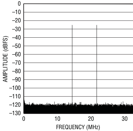
LTC2215 64k Point 2-Tone FFT, f_{IN} = 14.25\text{MHz} and 21.5\text{MHz} , -25dBFS, Dither "On"
