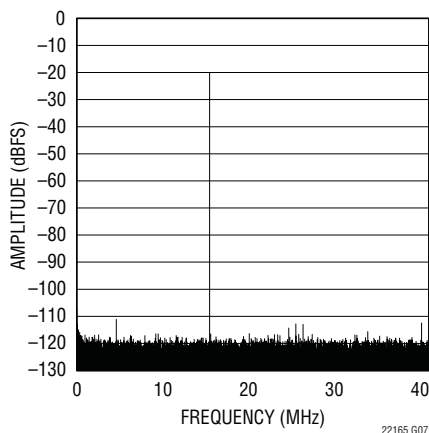
LTC2216 64k Point FFT, f_{IN} = 15.1\text{MHz} , -20dBFS, Dither "Off"
