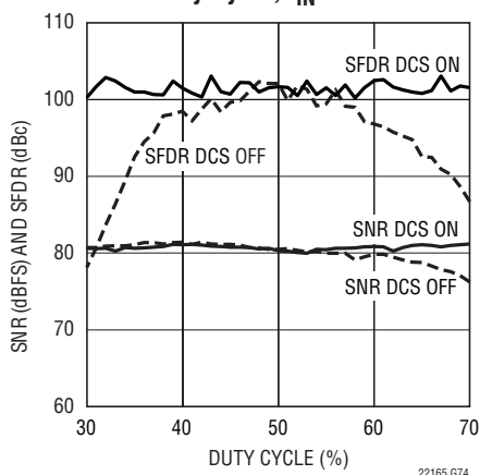
LTC2215 SNR and SFDR vs Clock Duty Cycle, f_{IN} = 5.2\text{MHz}
