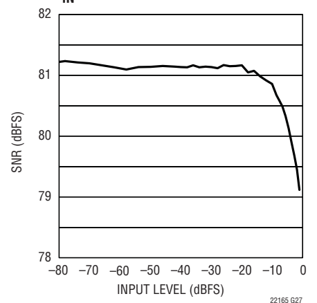
LTC2216 SNR vs Input Level, f_{IN} = 140.5\text{MHz}
