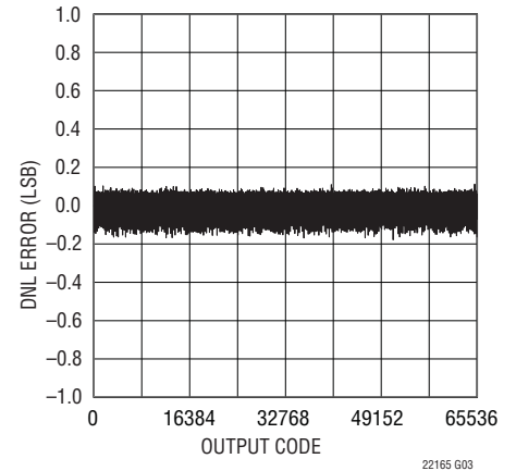
LTC2216 Differential Nonlinearity (DNL) vs Output Code
