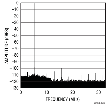
LTC2215 64k Point FFT, f_{IN} = 70.2\text{MHz} , -1dBFS
