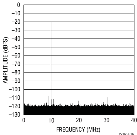
LTC2216 64k Point FFT, f_{IN} = 70.1\text{MHz} , -20dBFS, Dither "Off"
