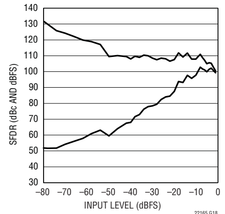
LTC2216 SFDR vs Input Level, f_{IN} = 70.5\text{MHz} , Dither "Off"
