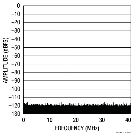
LTC2216 64k Point FFT, f_{IN} = 15.1\text{MHz} , -20dBFS, Dither "On"
