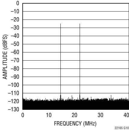
LTC2216 64k Point 2-Tone FFT, f_{IN} = 14.25\text{MHz} and 21.5\text{MHz} , -25dBFS, Dither "On"
