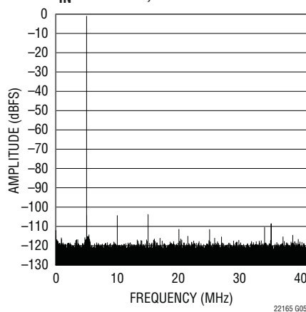
LTC2216 64k Point FFT, f_{IN} = 4.9\text{MHz} , -1dBFS
