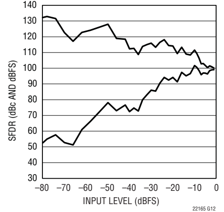
LTC2216 SFDR vs Input Level, f_{IN} = 15.2\text{MHz} , Dither "On"
