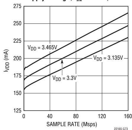
LTC2215 I_{VDD} vs Sample Rate and Supply Voltage, f_{IN} = 5\text{MHz} , -1\text{dBFS}
