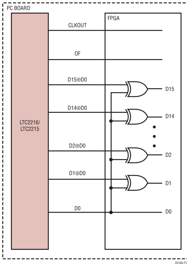
Figure 15. Descrambling a Scrambled Digital Output
