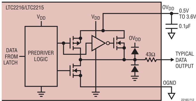
Figure 12. Equivalent Circuit for a Digital Output Buffer
