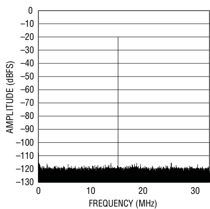
LTC2215 64k Point FFT, f_{IN} = 15.1\text{MHz} , -20dBFS, Dither "On"
