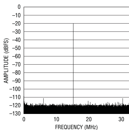
LTC2215 64k Point FFT, f_{IN} = 15.1\text{MHz} , -20dBFS, Dither "Off"
