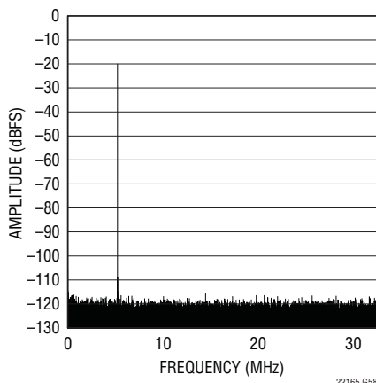
LTC2215 64k Point FFT, f_{IN} = 70.1\text{MHz} , -20dBFS, Dither "On"
