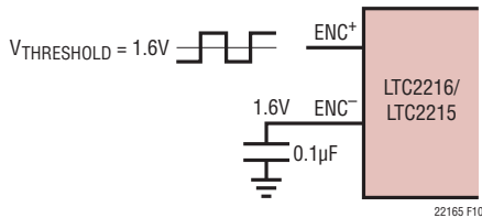
Figure 10. Single-Ended ENC Drive, Not Recommended for Low Jitter
