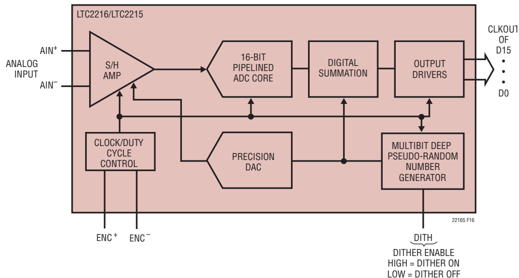
Figure 16. Functional Equivalent Block Diagram of Internal Dither Circuit
