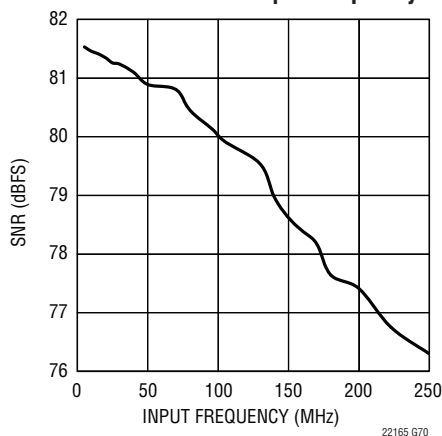
LTC2215 SNR vs Input Frequency
