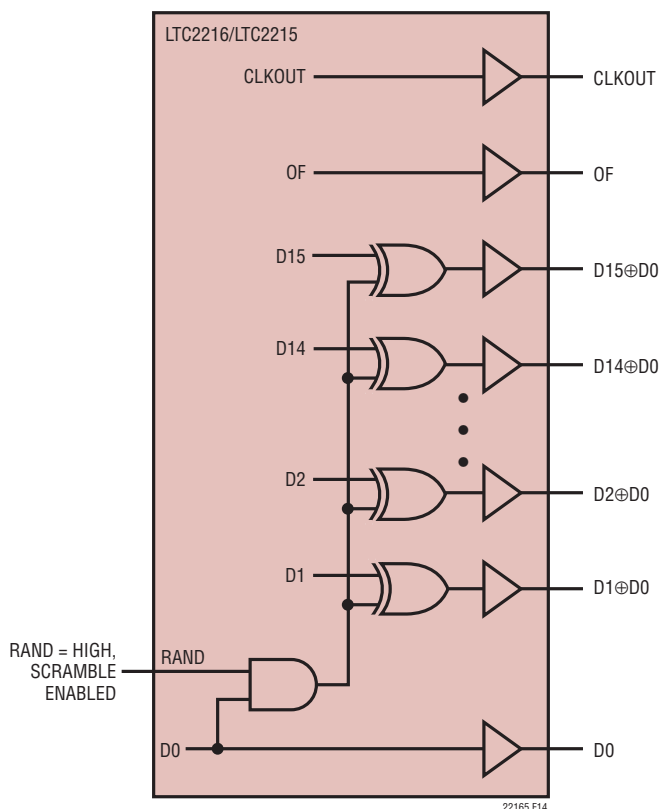
Figure 14. Functional Equivalent of Digital Output Randomizer
