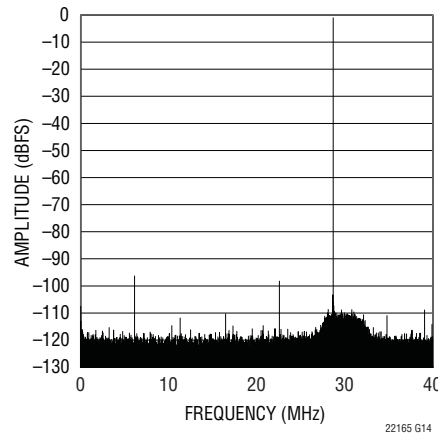
LTC2216 64k Point FFT, f_{IN} = 28.7\text{MHz} , -1dBFS
