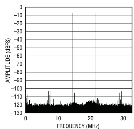
LTC2215 64k Point 2-Tone FFT, f_{IN} = 14.25\text{MHz} and 21.5\text{MHz} , -7dBFS
