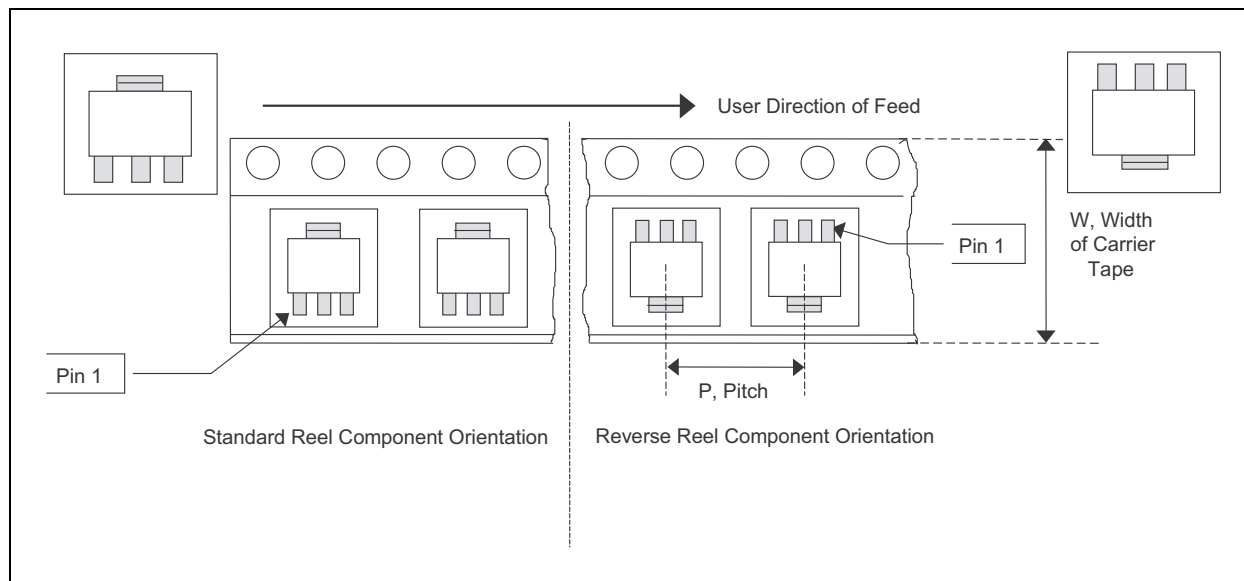
FIGURE 5-4: SOT-89 DEVICES
